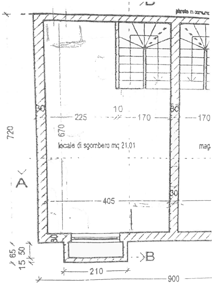
Pianta piano intero
